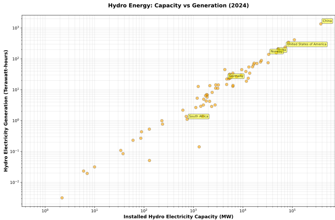
Figure 26: Comparison of installed hydro electricity capacity and generation.
