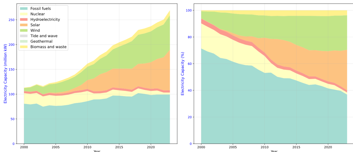
Figure 55: Electricity capacity installation in Germany.
