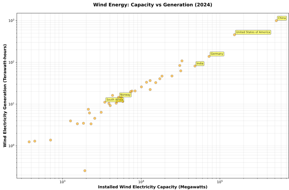
Figure 25: Comparison of installed wind electricity capacity and generation.
